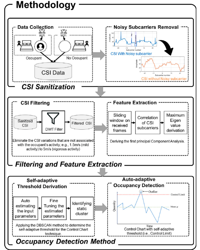
Fig. 1. High-level overview of the occupancy detection methodology.
