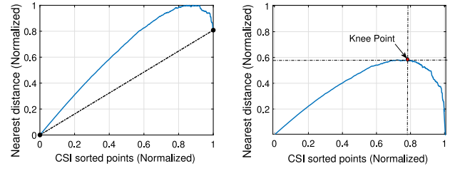
(a) Negative concavity of the sorted k-distance graph (normalized axis). (b) The knee point located at the maximum curvature of the sorted data points.
