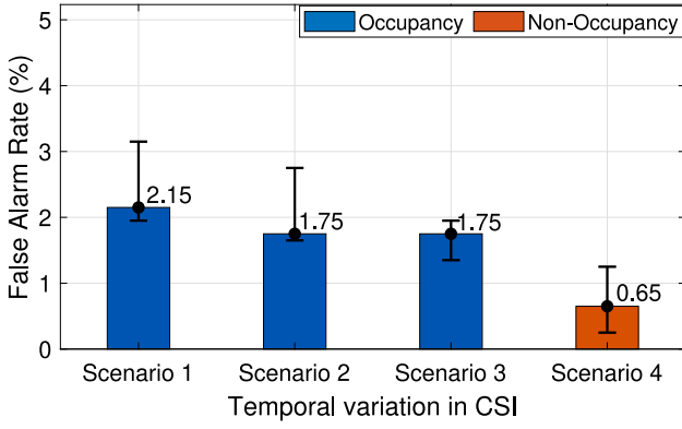
Fig. 5. False Alarm Rate obtained with temporal variations in CSI.
