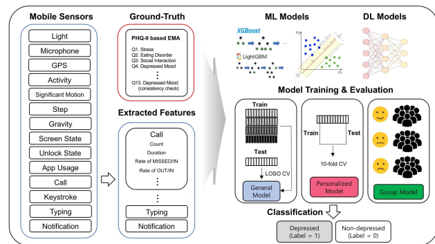
Fig. 1. STDD Data Processing Pipeline
