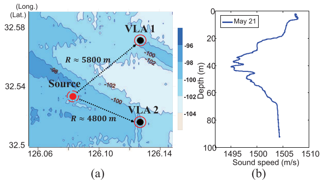
Fig. 3. System installation and measured oceanographic data near Jeju Island in [9]: (a) locations of the source and receivers with seafloor bathymetry; (b) an instance of the measured sound speed profile on May 21.
