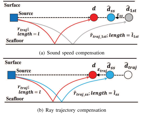
Fig. 1. Schematic diagram of the RAR algorithm.
