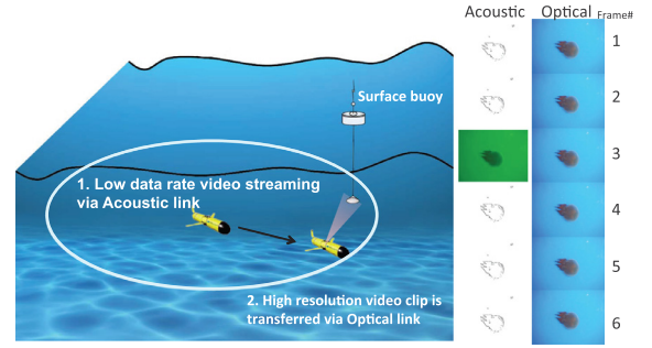
Fig. 2. Real-time video streaming via Acoustic/Optical.
