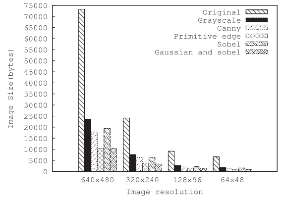
Fig. 5. Average file sizes for different image resolutions.
