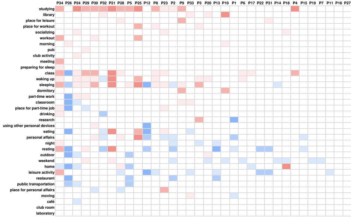
Fig. 2. The individual models were visualized to show the relationships between contexts and distraction level. Each column and row in the table indicates an individual participant and the context, respectively. Blue color means negative relation with perceived smartphone distraction (i.e., less distracting). Orange color denotes positive relation with perceived smartphone distraction (i.e., more distracting).
