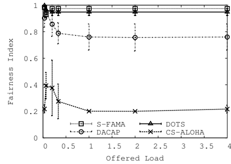
Fig. 14. Jain's Fairness Index for the four protocols
